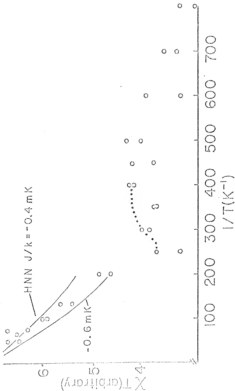
Fig. 13 \chi T plot of solid Helium three susceptibility.
